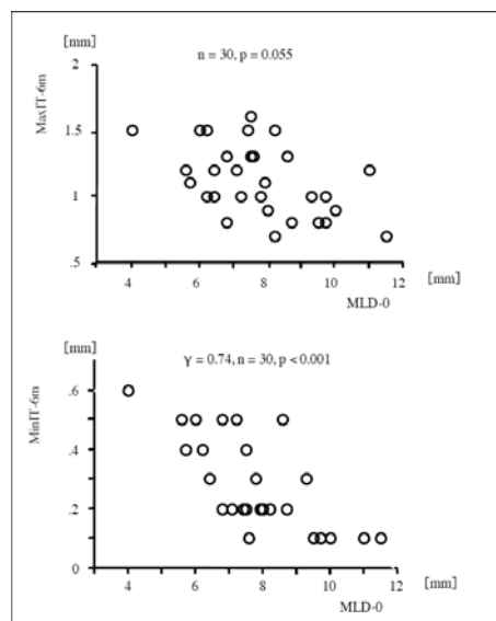
Figure 5. The relationship of MLD-0 to MaxIT-6m (upper panel) and to MiniIT-6m (lower panel).
